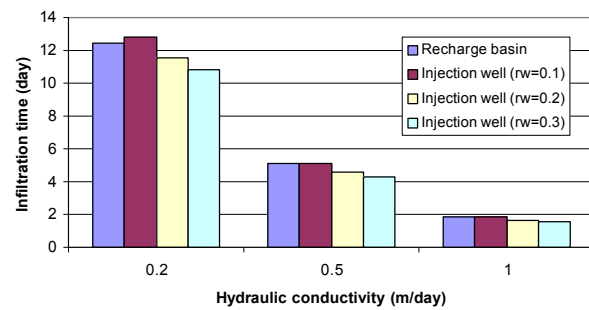
Fig. 9: Comparison between the infiltration time for recharge basin and injection recharge well
