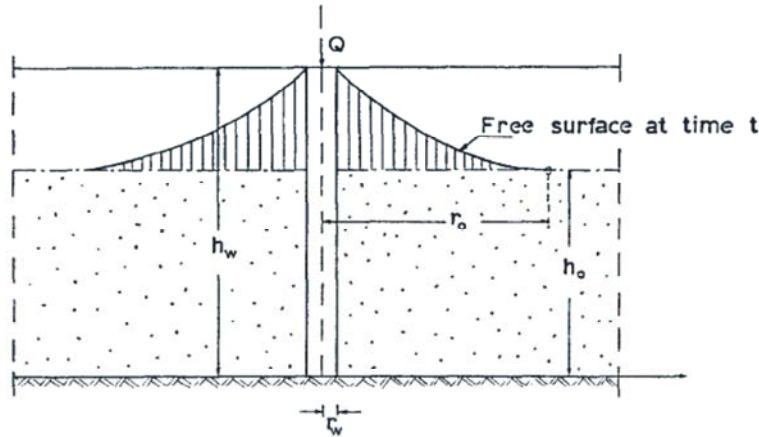
Fig. 3: Schematic sketch of recharge well
