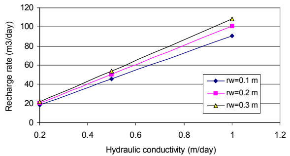
Fig. 8: Variation of recharge rate with hydraulic conductivity for injection recharge wells at different wells radius
