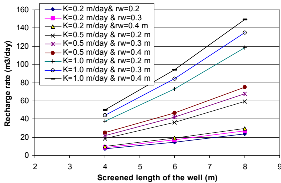
Fig. 6: Variation of recharge rate will screened length of Vadose zone recharge well at different values of hydraulic conductivity and well radius
