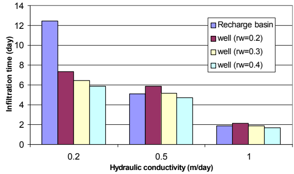
Fig. 7: Comparison between the infiltration time for recharge basin and vadose zone well
