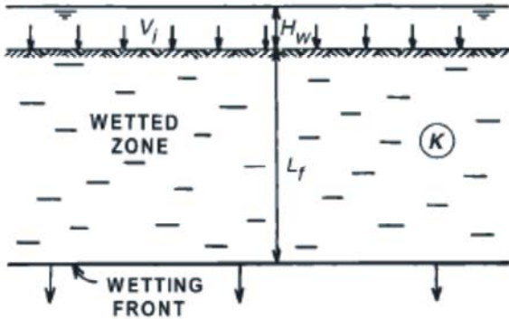
Fig. 1: Schematic diagram for the variables used in Eqn.(1)
