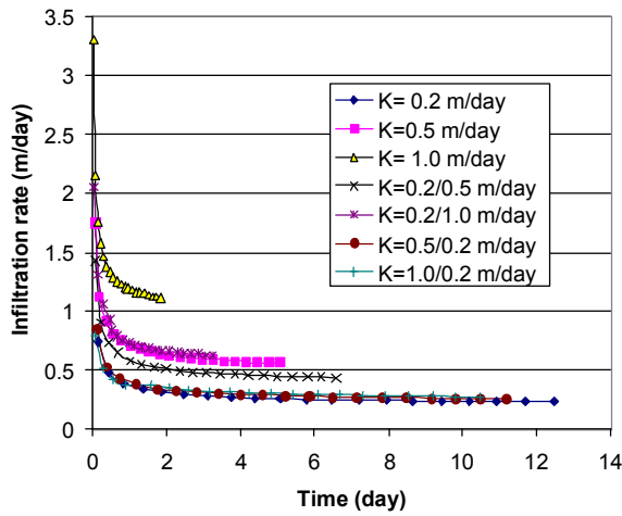
Fig. 5: Variation of infiltration rate with time at different values of saturated hydraulic conductivity
