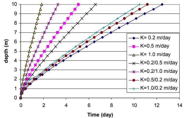
Fig. 4: Advance wetting depth versus time at different saturated hydraulic conductivity
