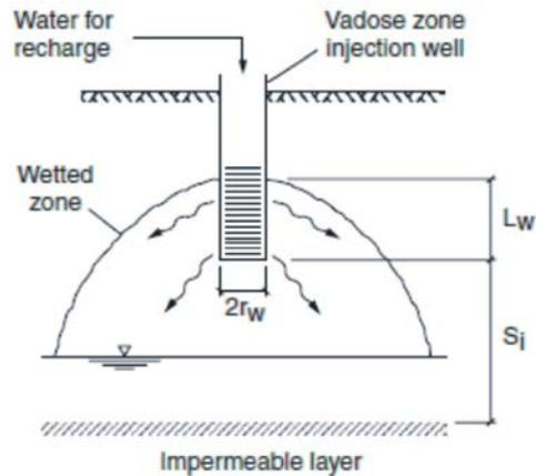
Fig. 2: Schematic of vadose zone injection well wetted zone
